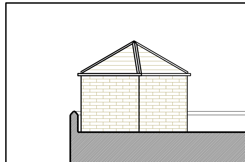
West Elevation - Proposed
