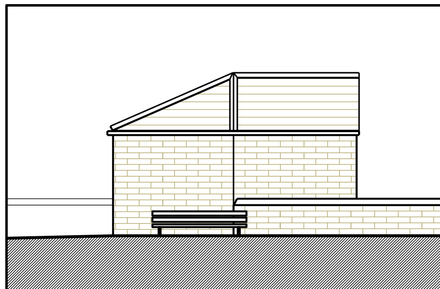
South Elevation - Proposed
