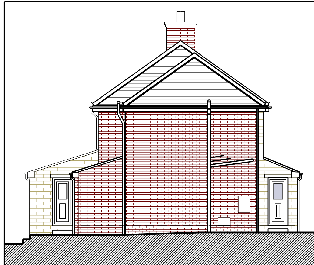
West Elevation
