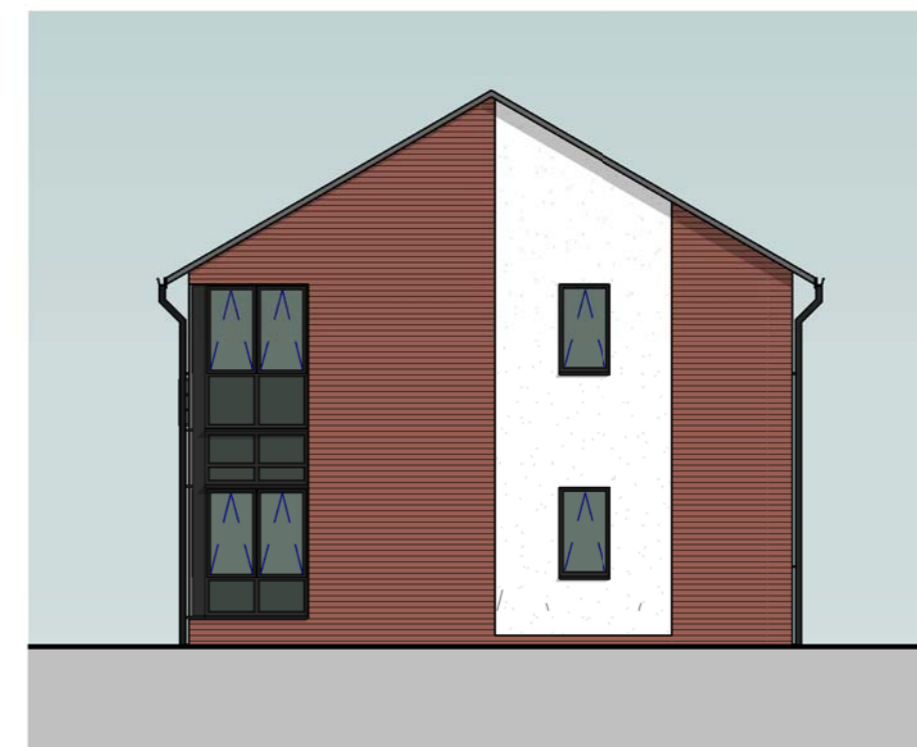
Plot 4 Side / North Elevation 1 : 100
