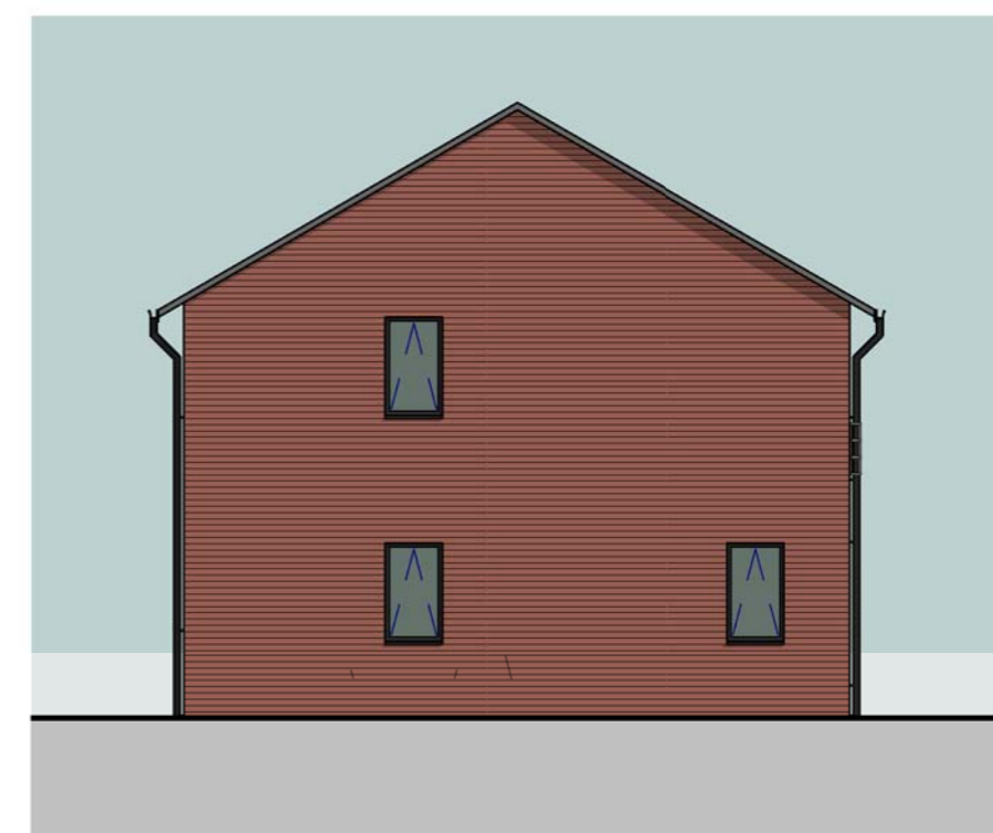
Plot 5 Side / South Elevation 1 : 100
