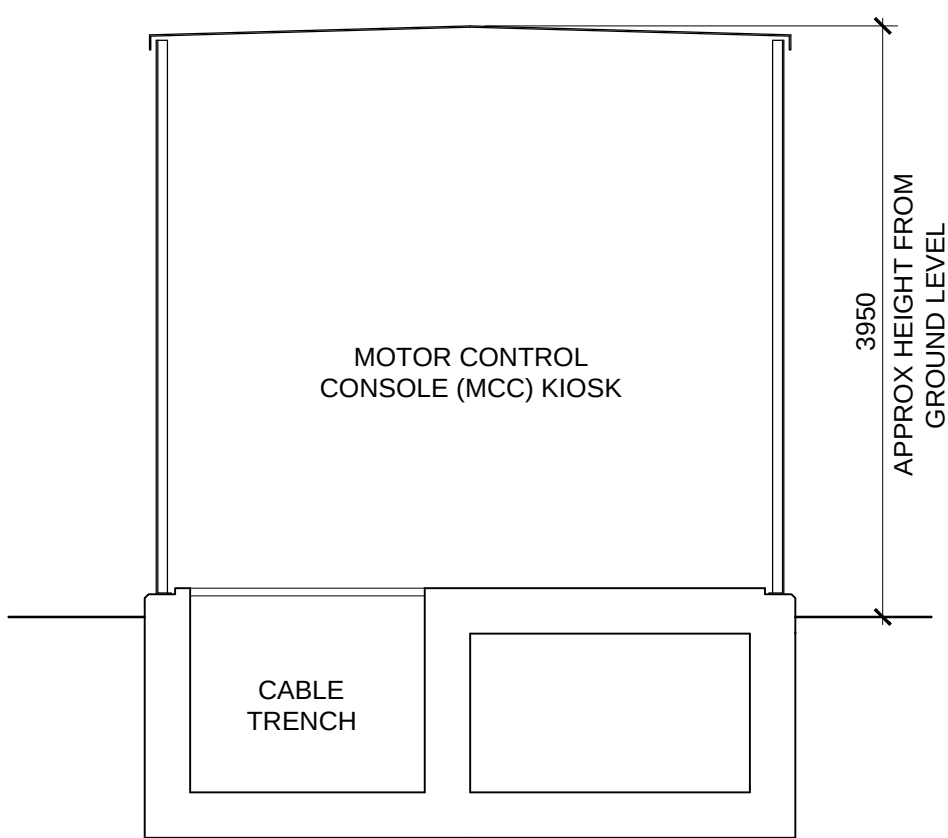
SECTION A SCALE 1:50
