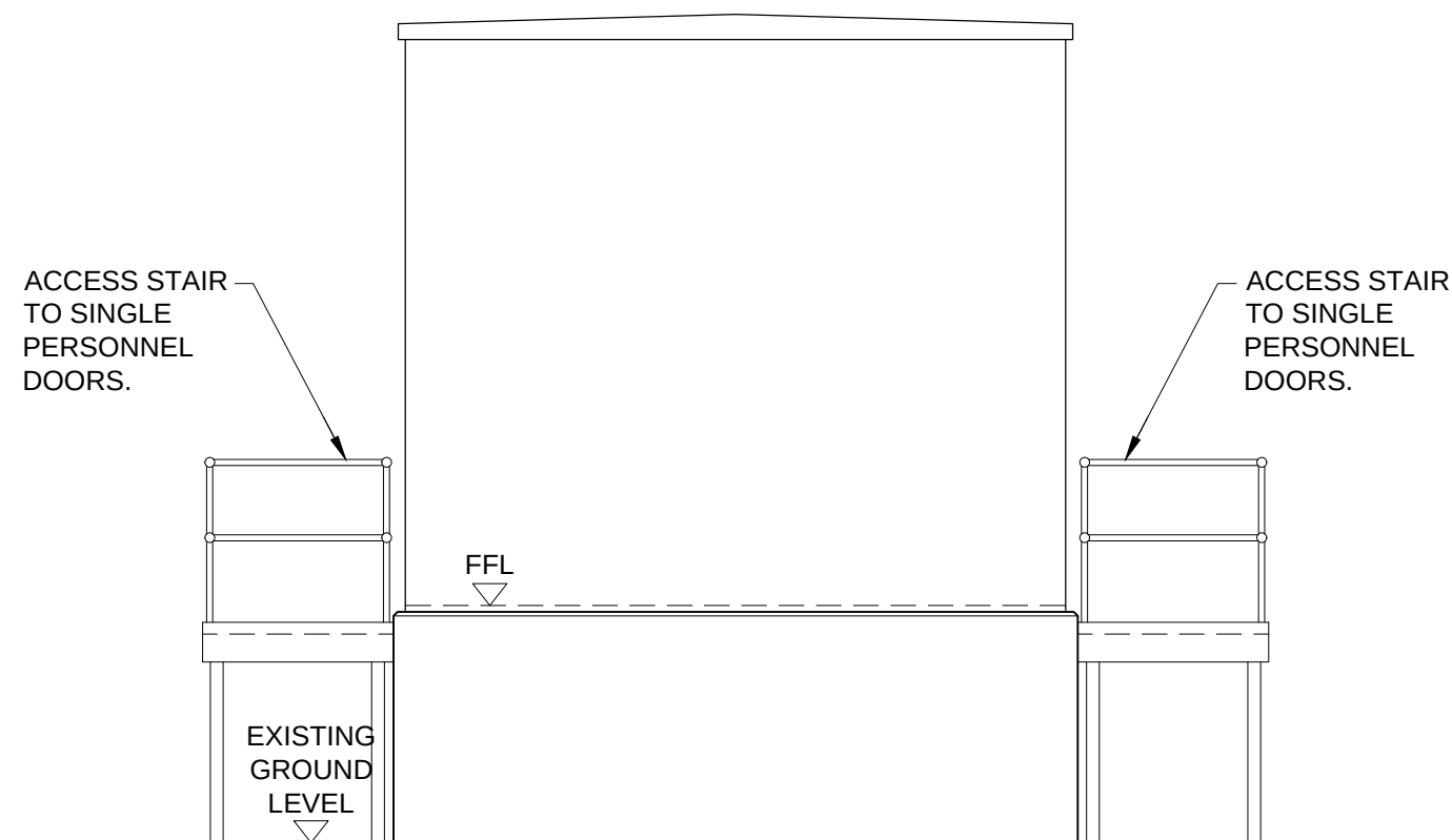
ELEVATION C SCALE 1:50
