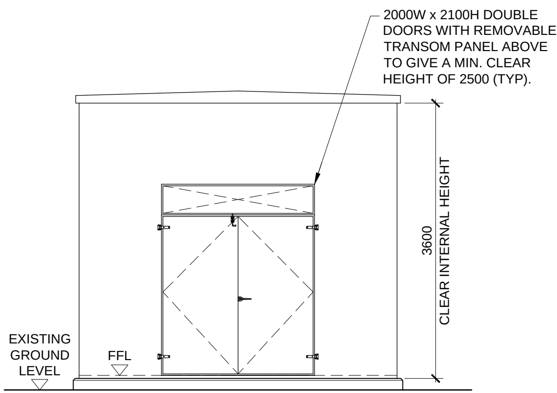
ELEVATION A SCALE 1:50
