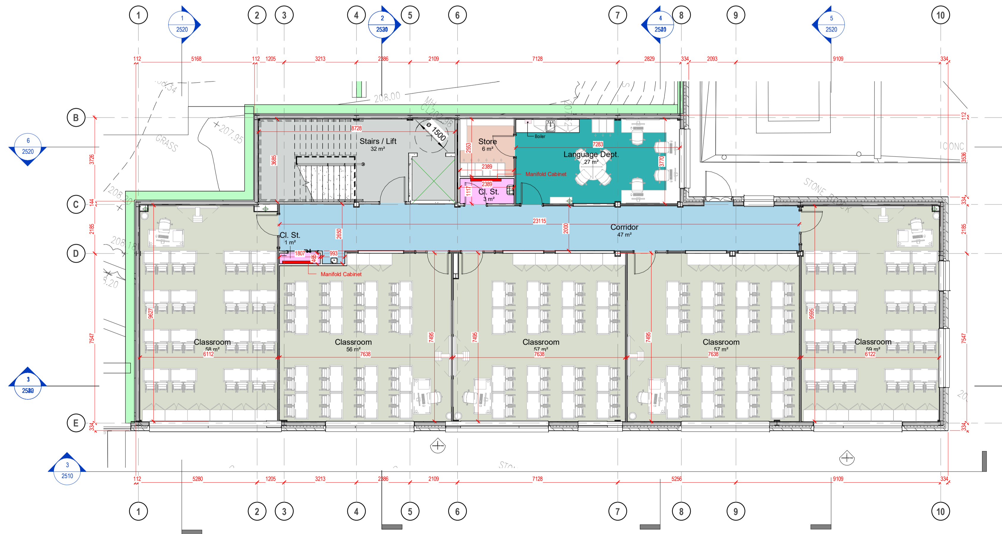
1 Level 1 1:100 Ref Sheet: 0301
