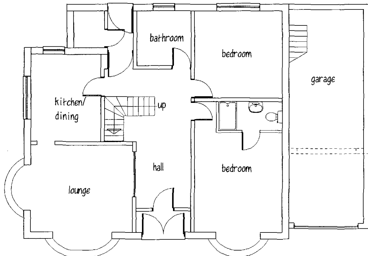
GROUND FLOOR
