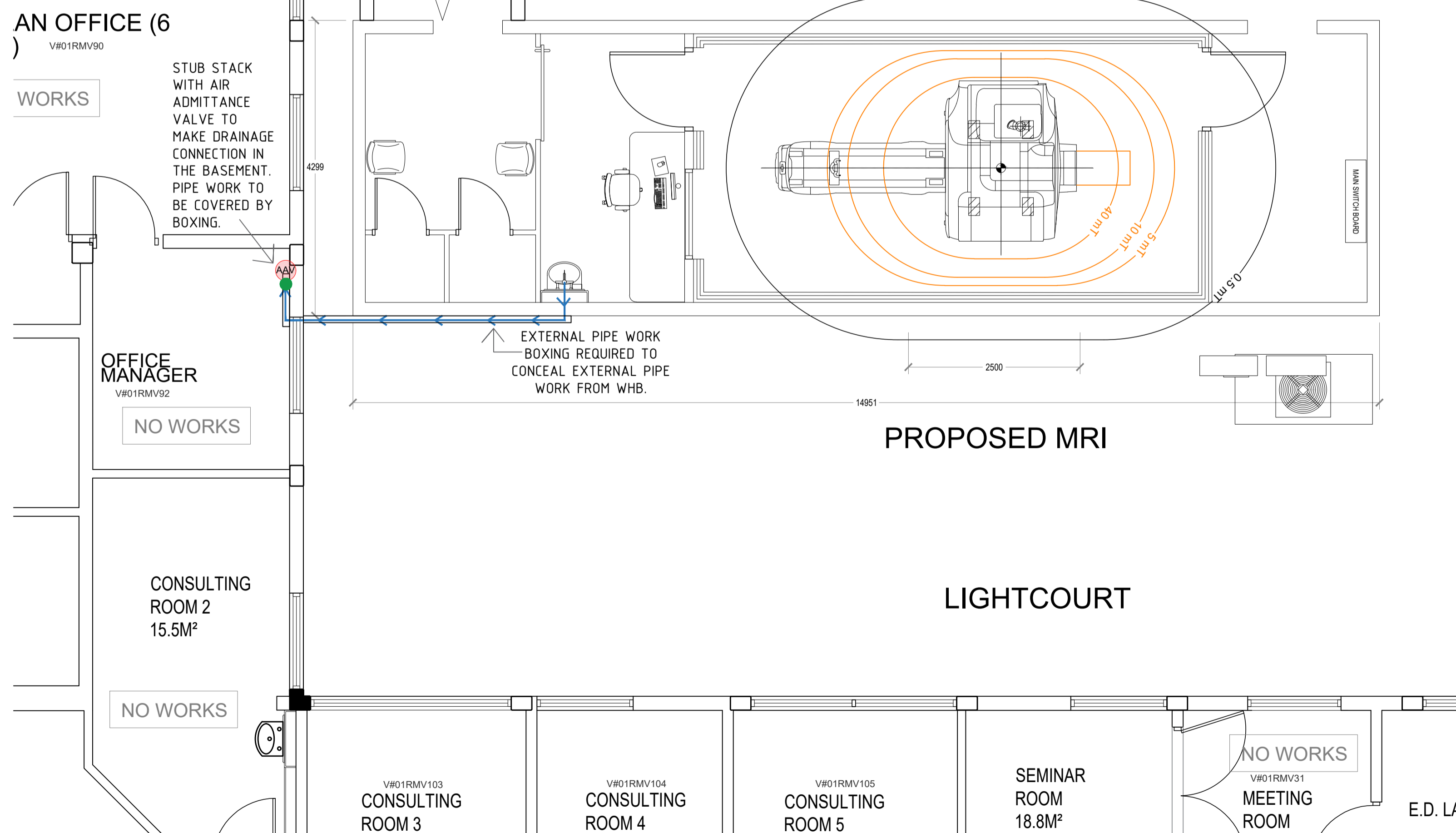
PROPOSED DRAINAGE PLAN 1:50
