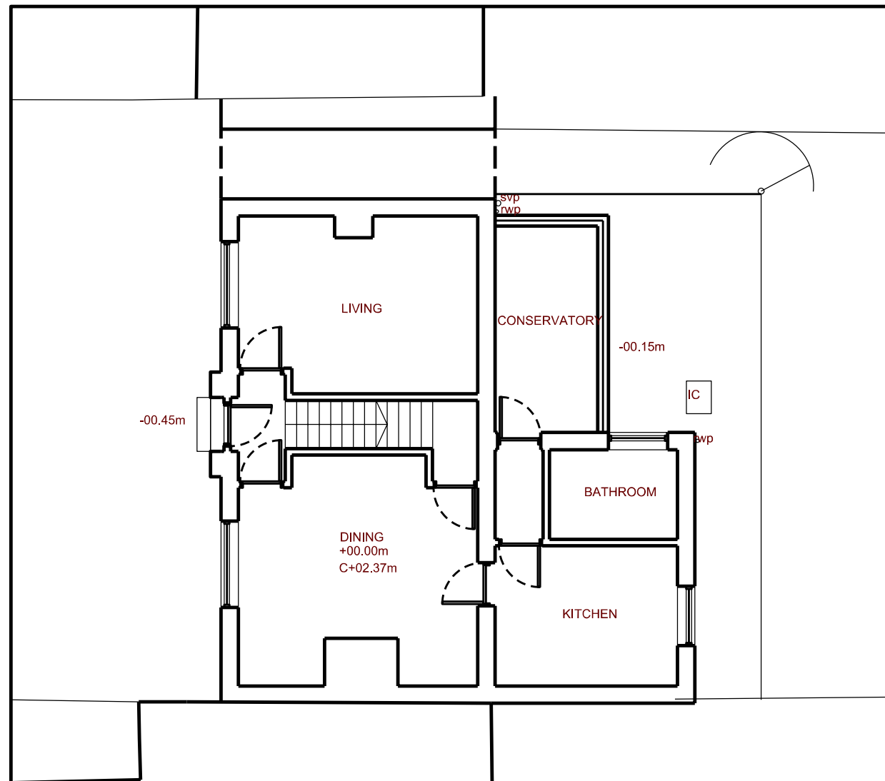
Ground Floor Plan - Existing
