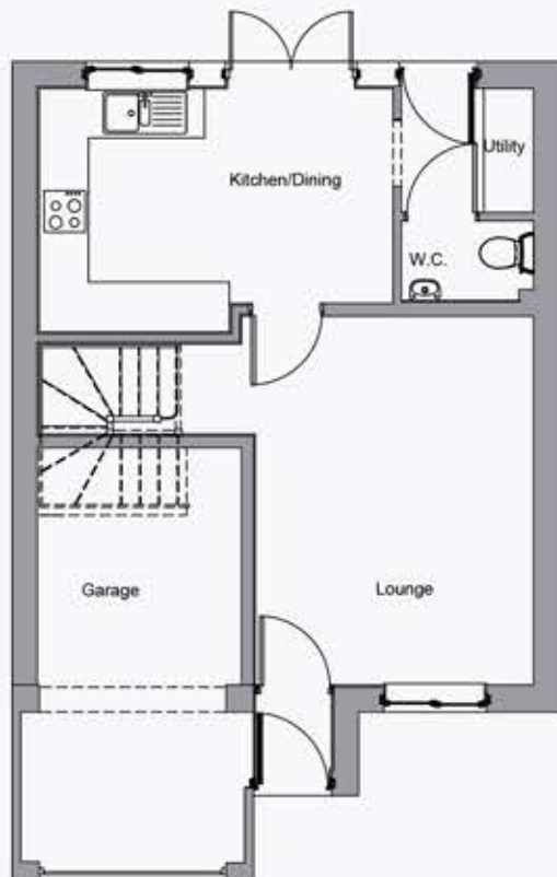
Alderton Stone GROUND FLOOR PLAN
