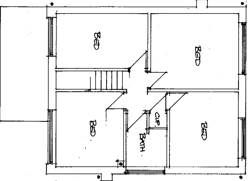
FIRST 1:100
