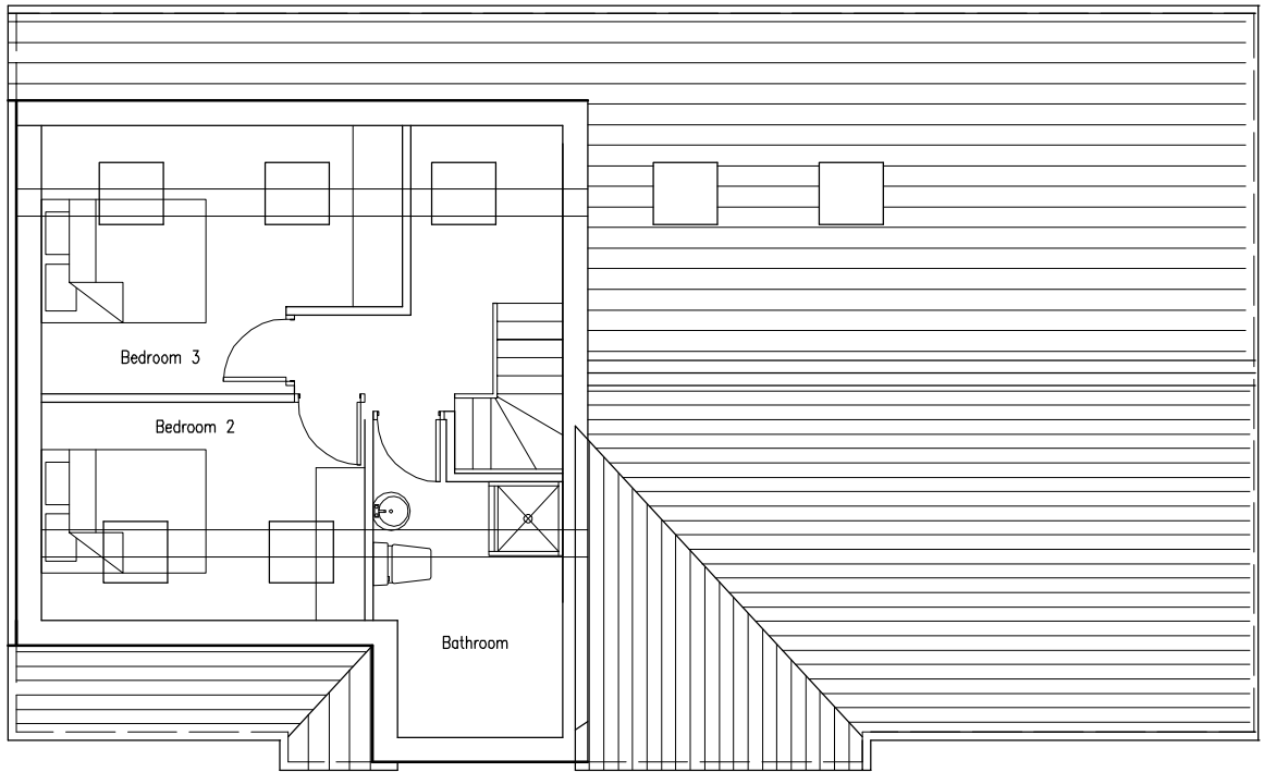
Second Floor Layout
