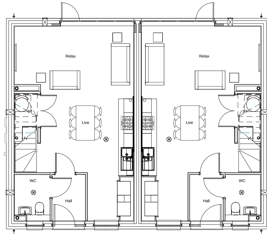
GROUND FLOOR PLAN HAMILTON
