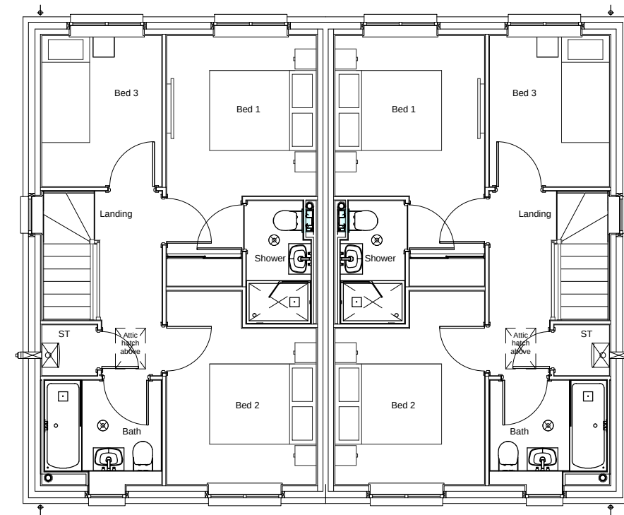
FIRST FLOOR PLAN HAMILTON
