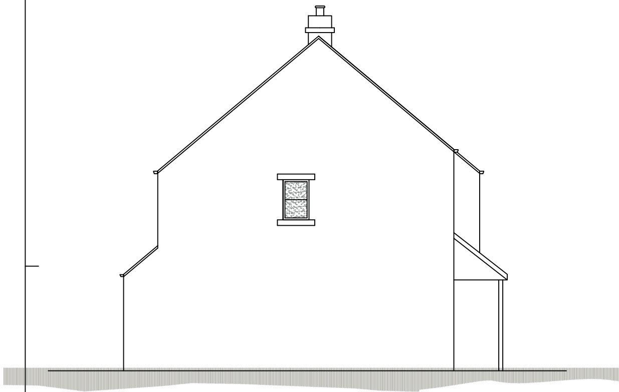
SIDE ELEVATION
