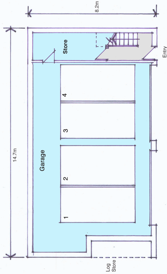
Ground level Plan
