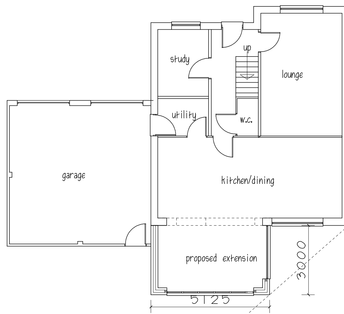
GROUND FLOOR
