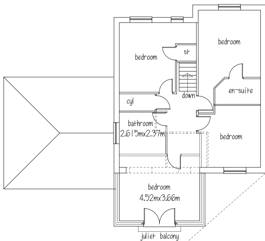
FIRST FLOOR
