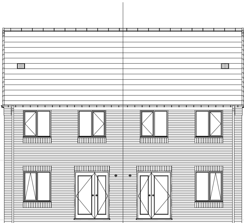
REAR ELEVATION
