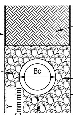
CLASS S BED AND SURROUND
