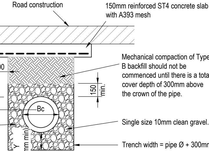
CLASS S WITH CONCRETE PROTECTION SLAB
