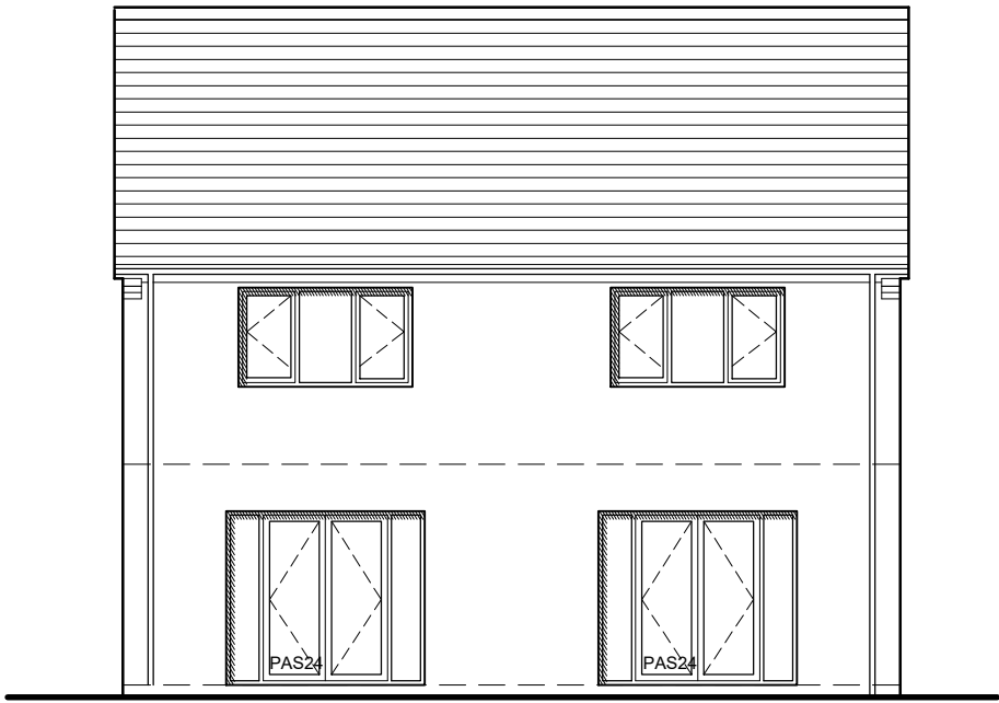
REAR ELEVATION
