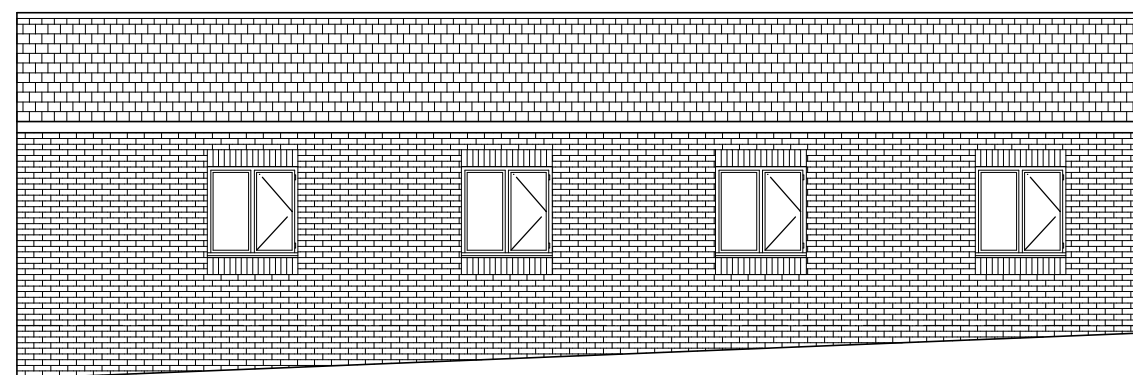
REAR ELEVATION (facing beacon close)
