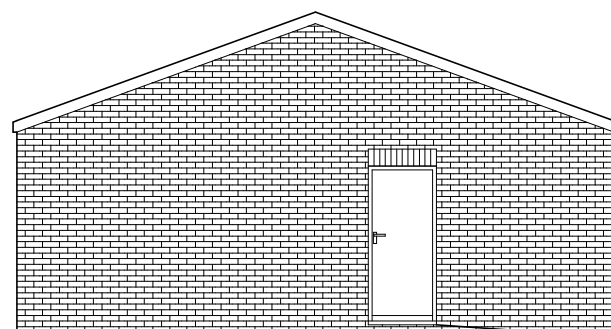
SIDE ELEVATION
