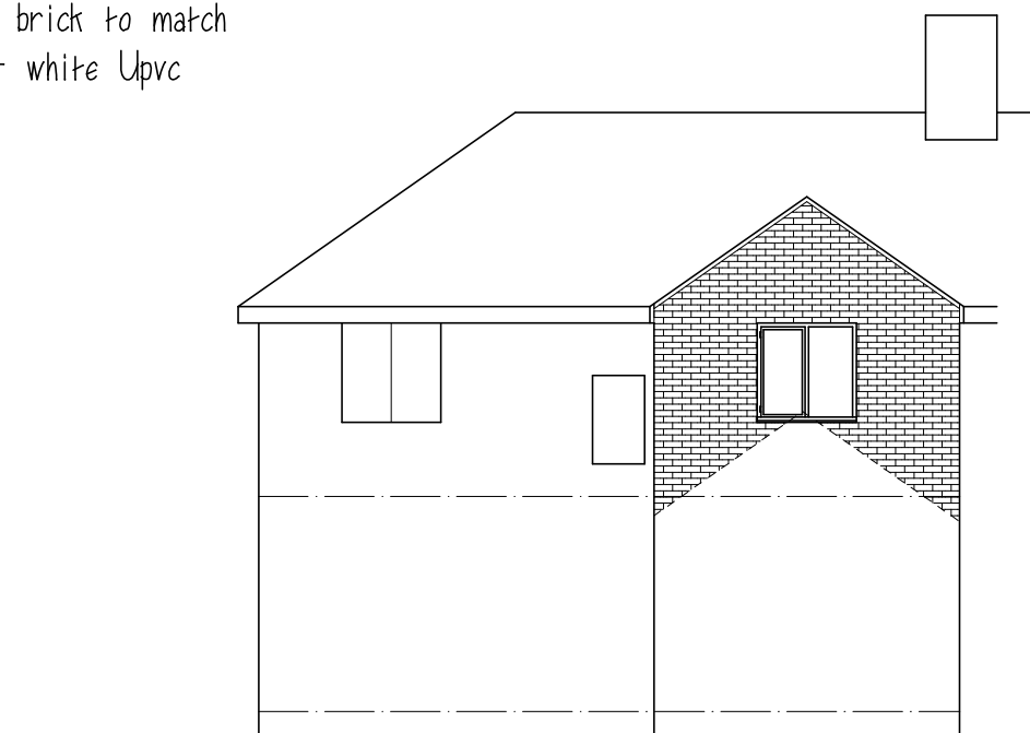
REAR ELEVATION
