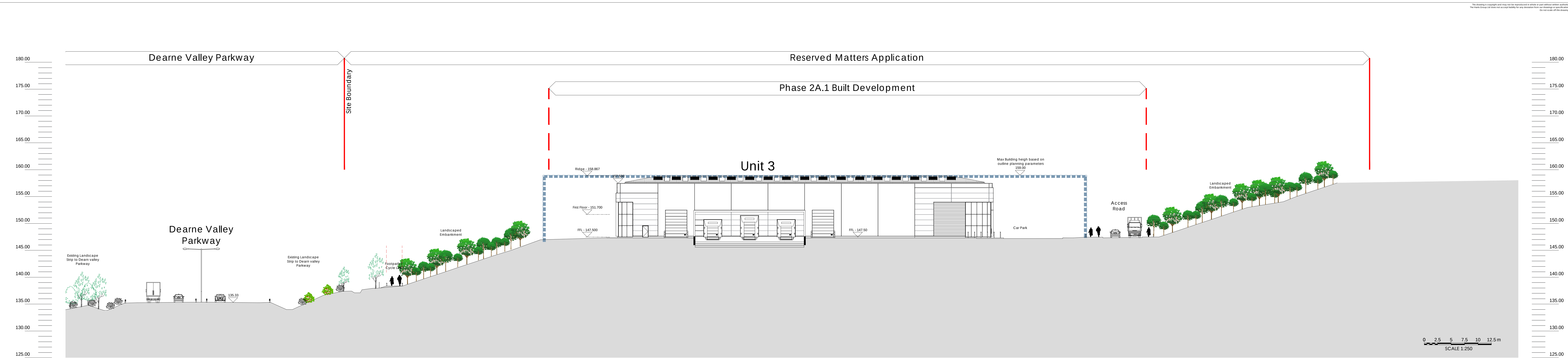
Section 3 - After completion of the development - 1:500
