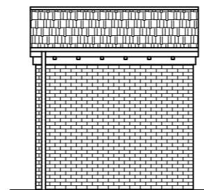
PROPOSED END ELEVATION SCALE 1:100 AT A3
