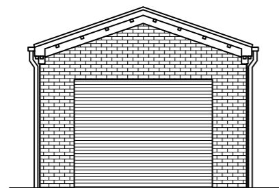
PROPOSED FRONT ELEVATION SCALE 1:100 AT A3
