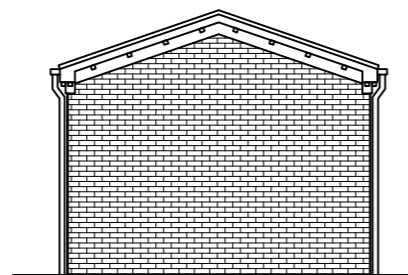
PROPOSED REAR ELEVATION SCALE 1:100 AT A3
