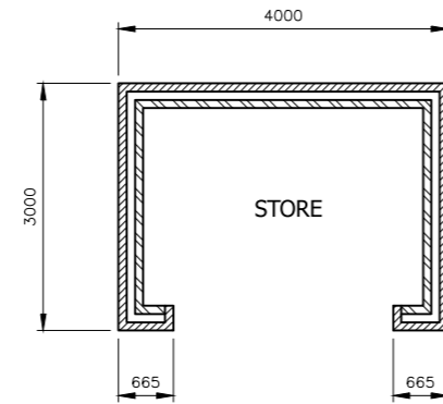
PROPOSED PLAN SCALE 1:100 AT A3
