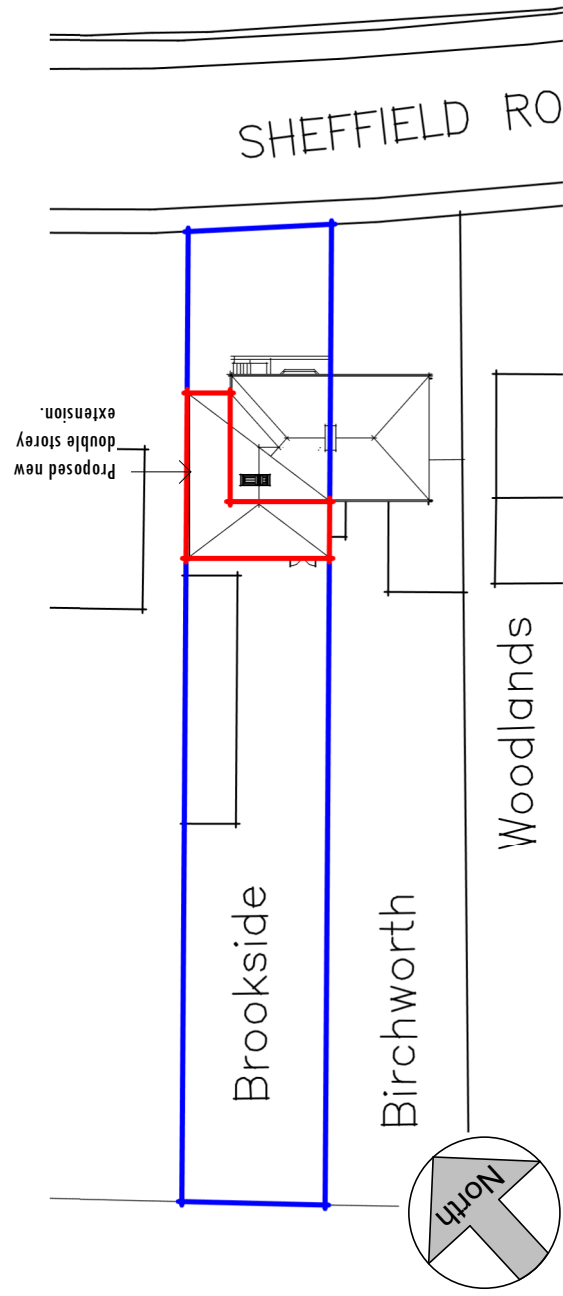
Proposed Block Plan 1 : 500
