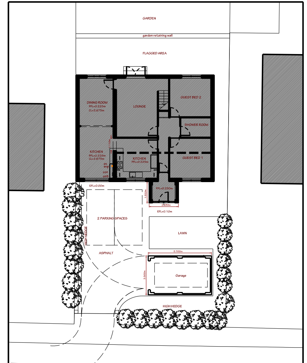
Site Plan - Proposed 1:200
