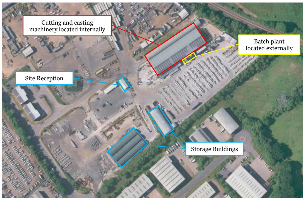
Figure 4.1: Development Layout
