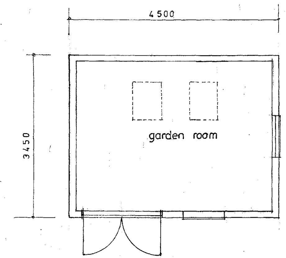
PLAN GARDEN ROOM TYPE 3 RHOMBUS
