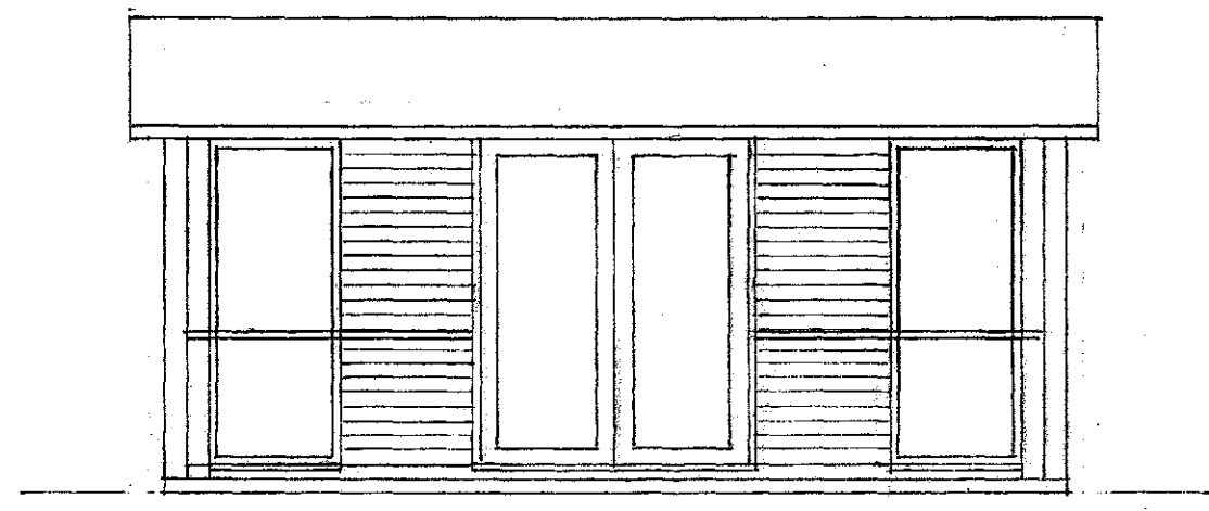
Front Elevation 2
