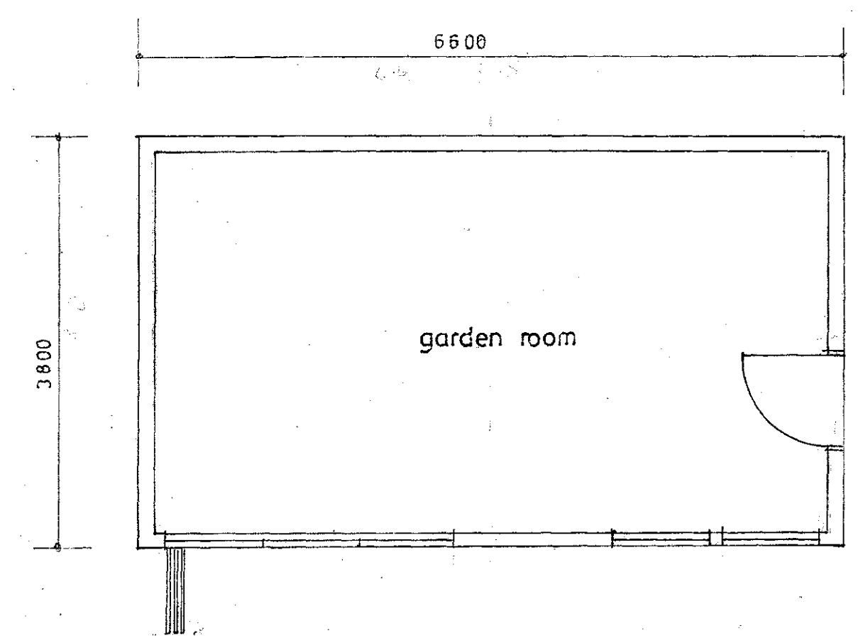
PLAN GARDEN ROOM TYPE 1 PRISMA
