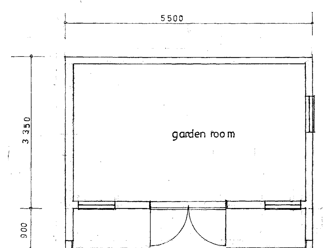
PLAN GARDEN ROOM TYPE 2 SCALENE
