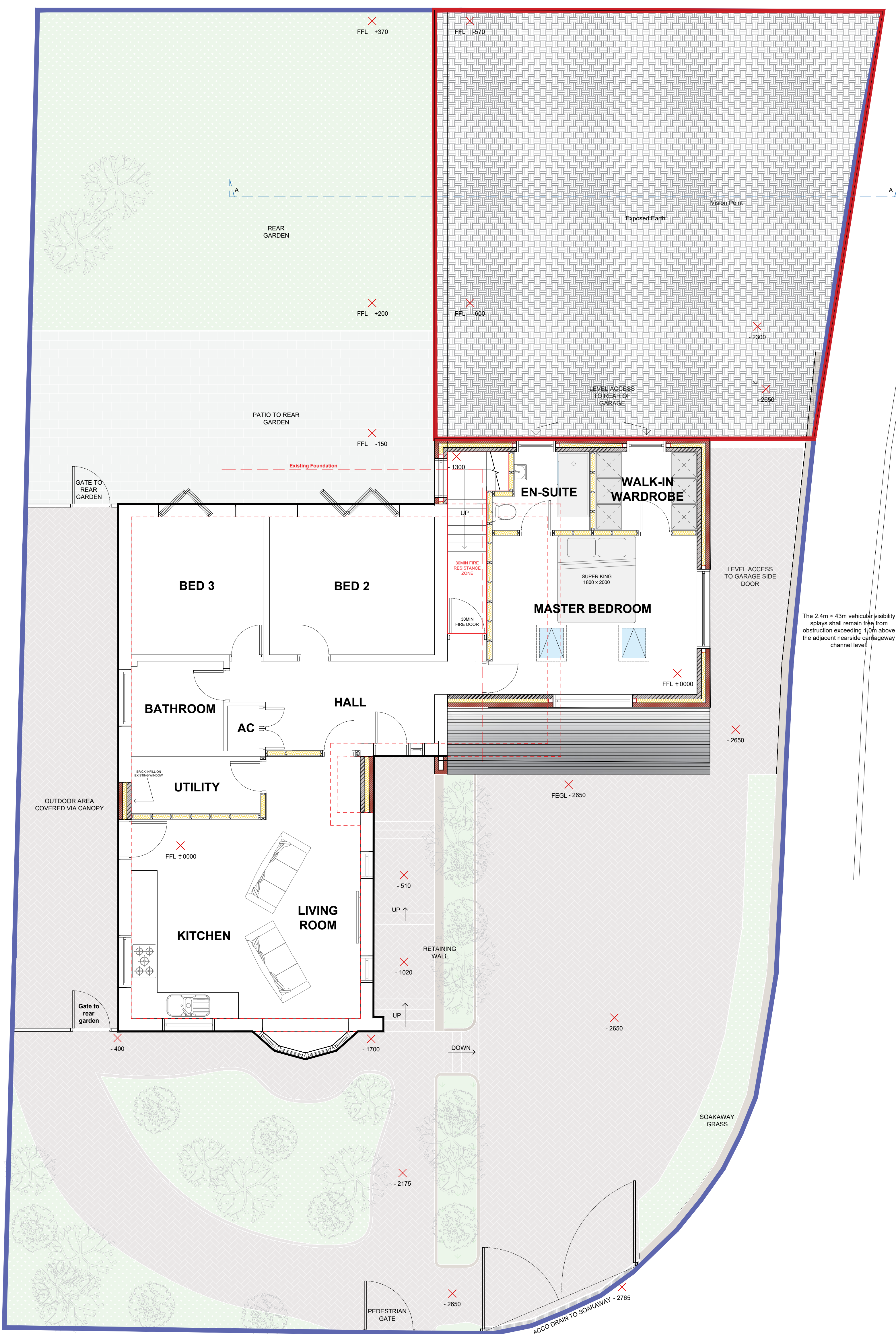
Proposed Plan Site / Block Plan Combined Scale 1:50
