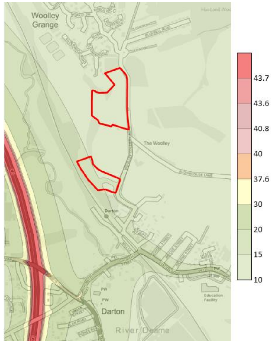
Figure 6-2. Total Long Term Annual Average Nitrogen Dioxide (NO 2 ) Concentration at Proposed Development (µg/m 3 )
