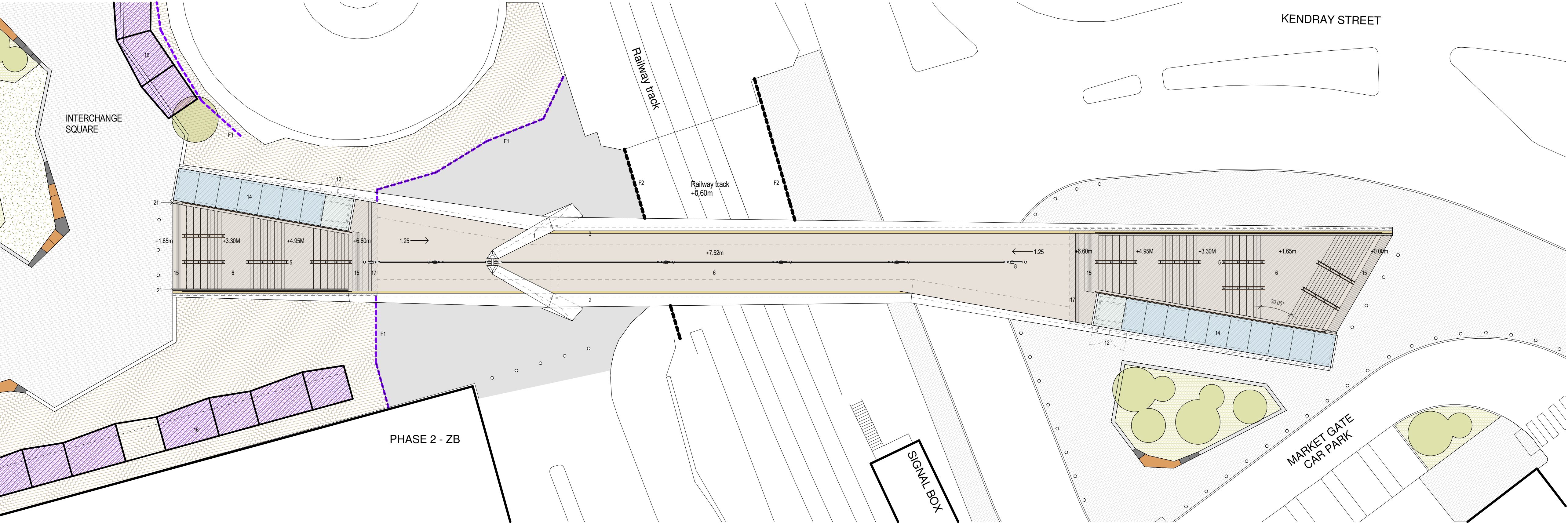
Bridge Deck and Pylon Plan 1:200
