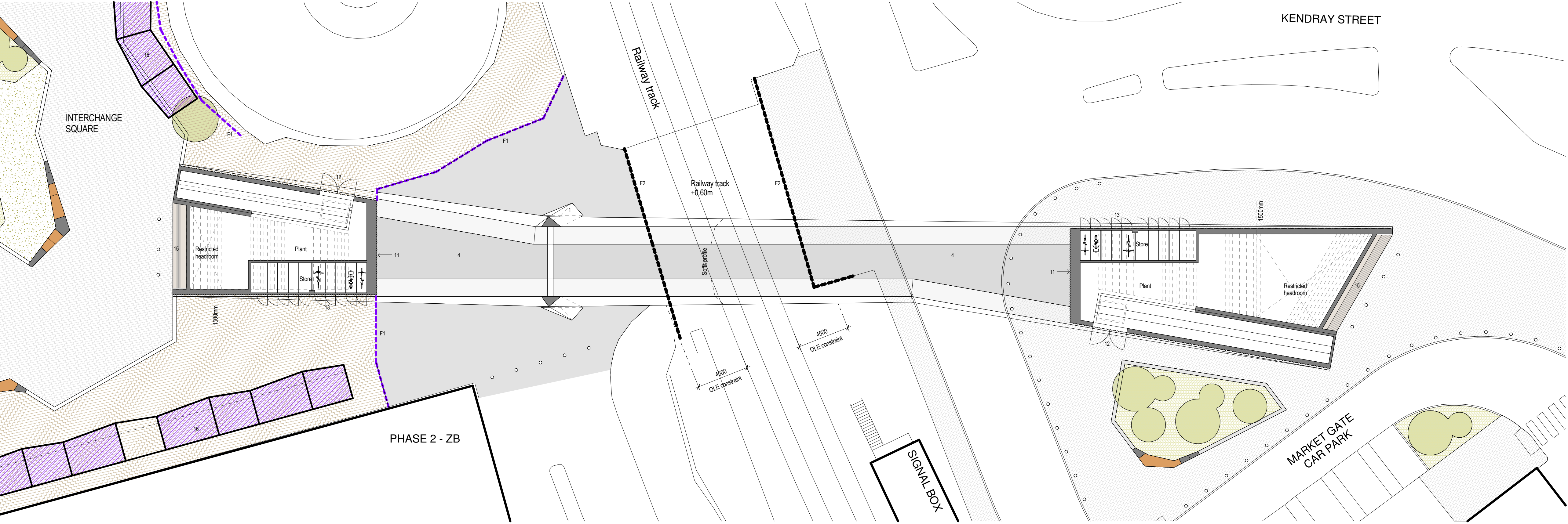
Reflected Bridge Soffit and Stairs undercroft Plan 1:200
