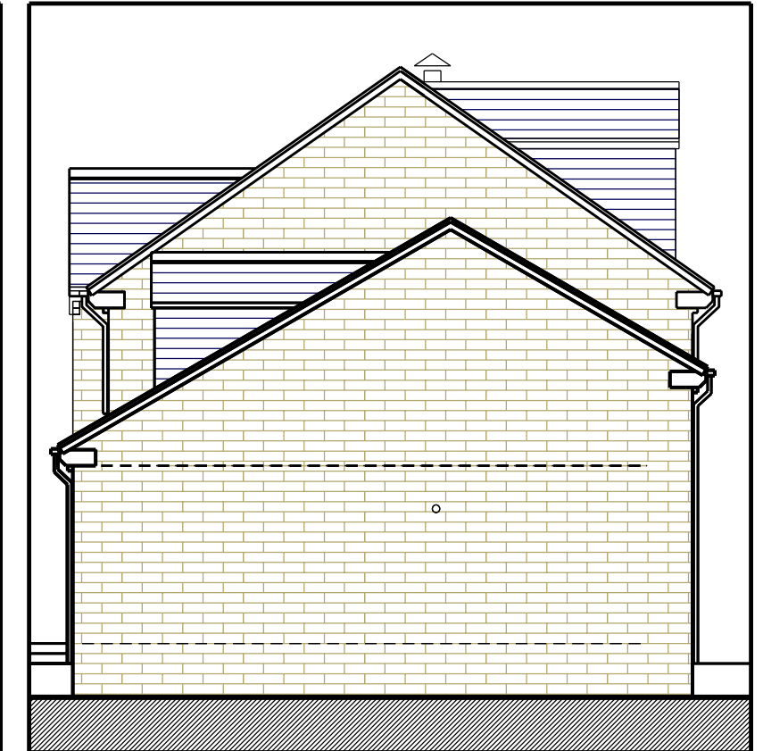
North Elevation
