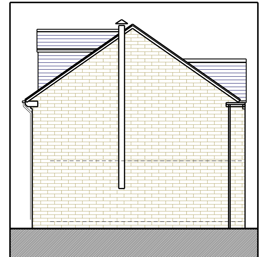
South Elevation
