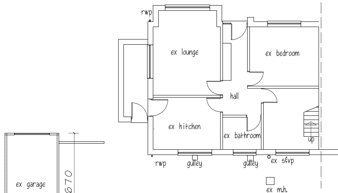
GROUND FLOOR
