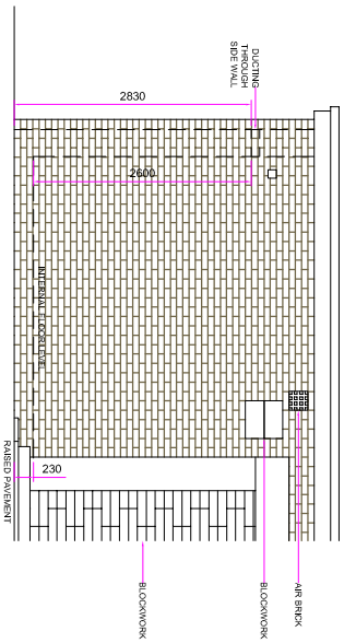
PROPOSED (PART) PLAN
