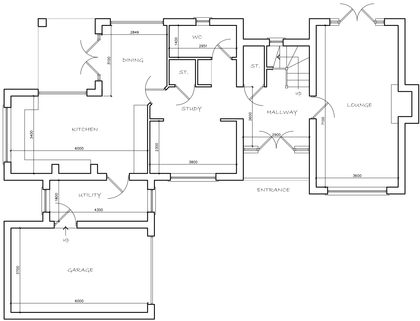
PLOT 1 - PROPOSED GROUND FLOOR PLAN SCALE - 1:100
