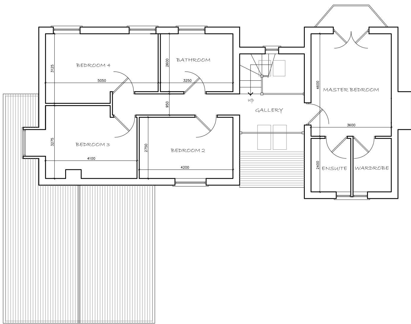
PLOT 1 - PROPOSED FIRST FLOOR PLAN SCALE - 1:100
