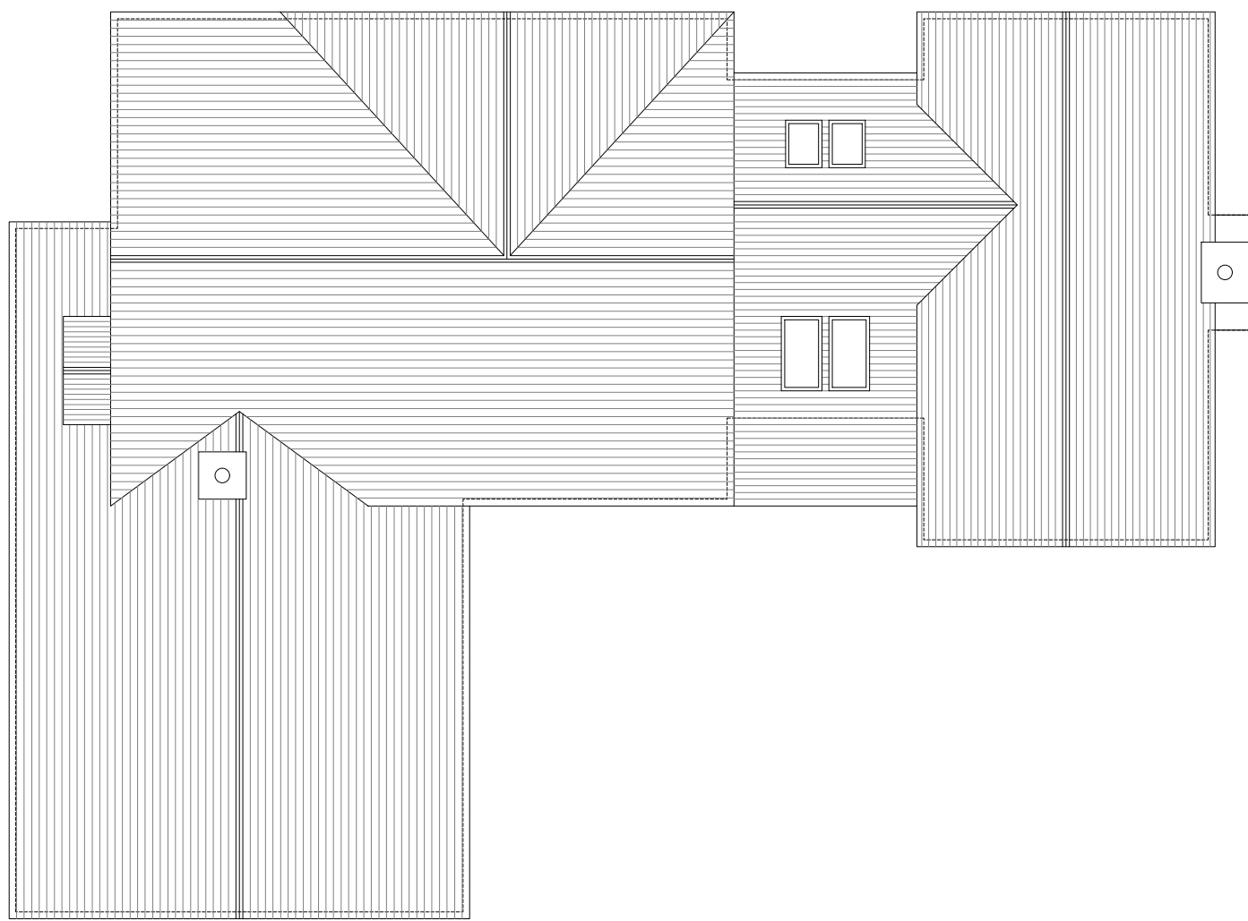
PLOT 1 - PROPOSED ROOF PLAN SCALE - 1:100
