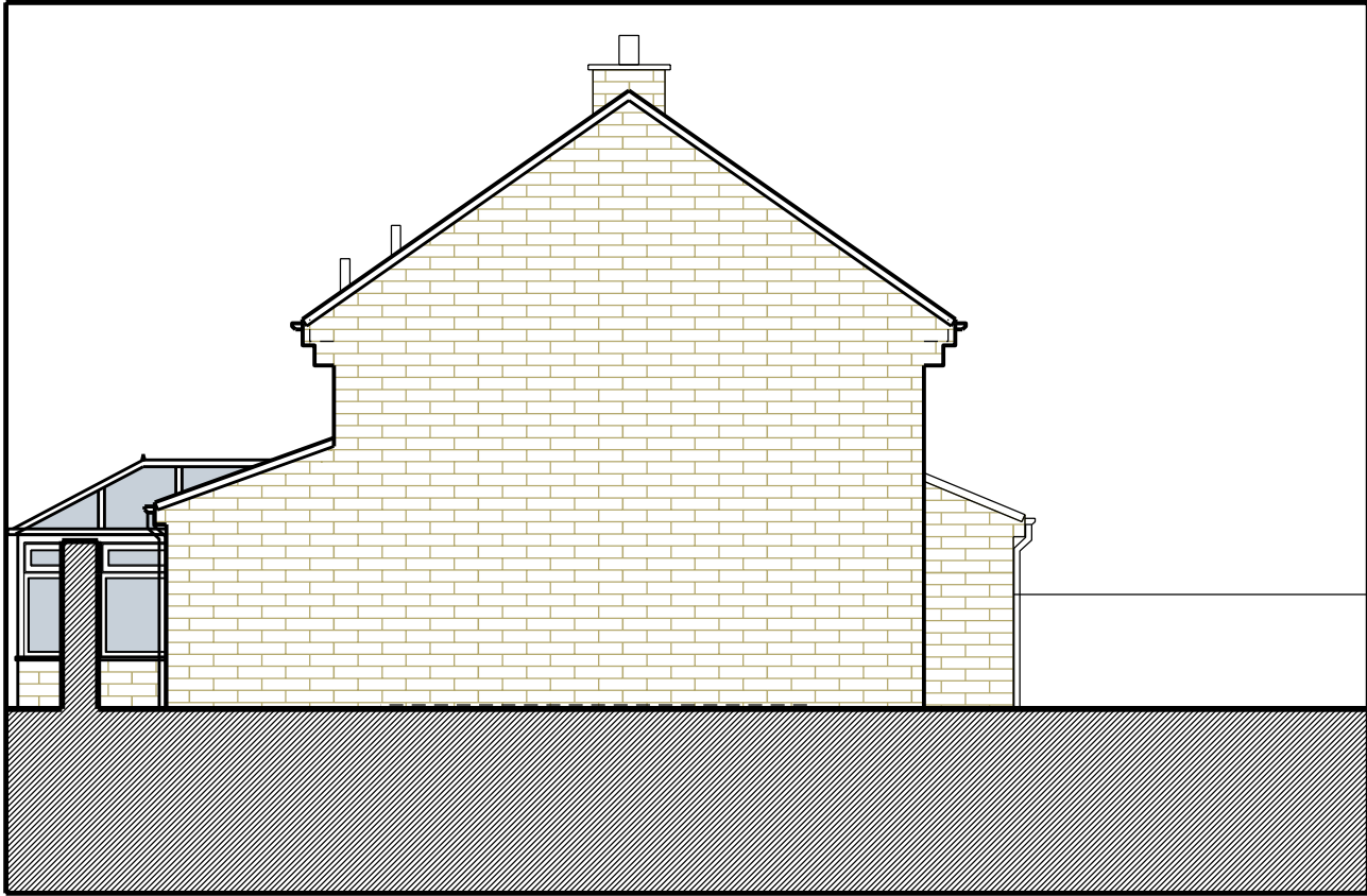
South Elevation - Proposed
