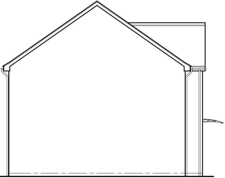
Side Elevation(as)
