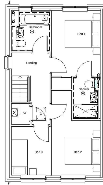
FIRST FLOOR PLAN Kilmingston
