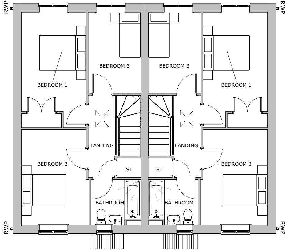
First Floor 1 : 100
