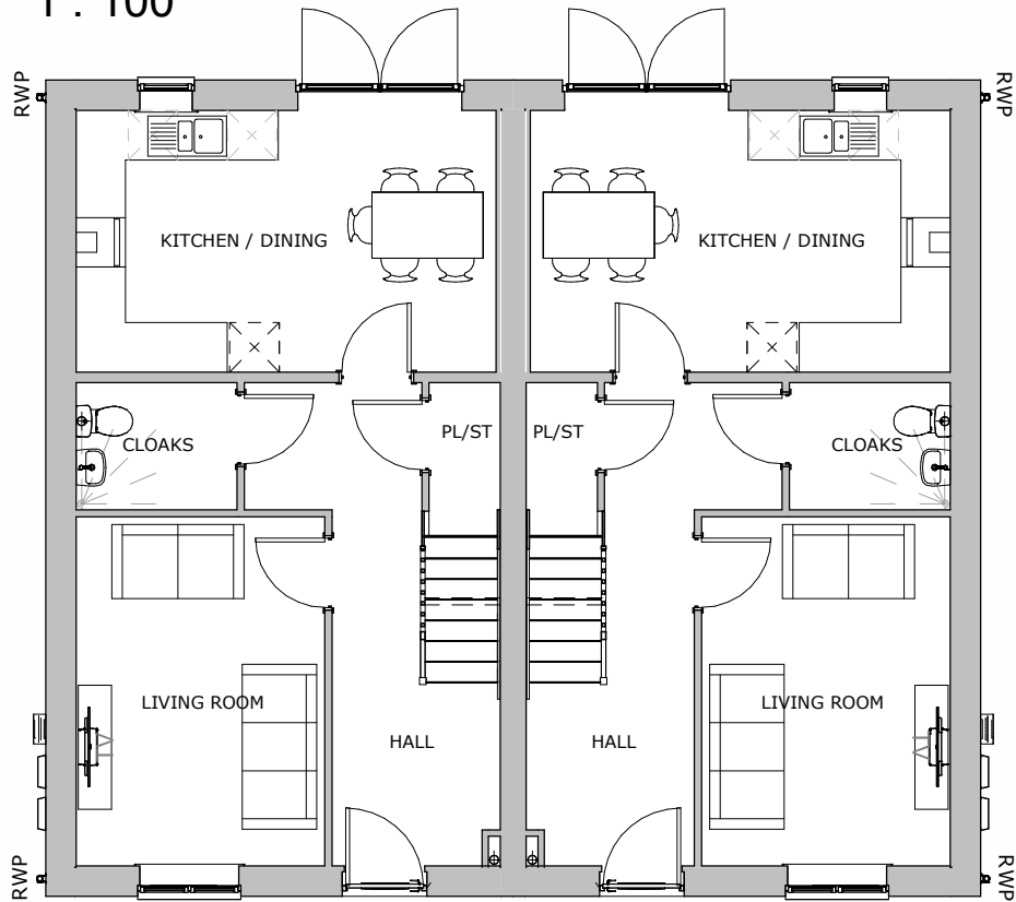
Ground Floor 1 : 100
