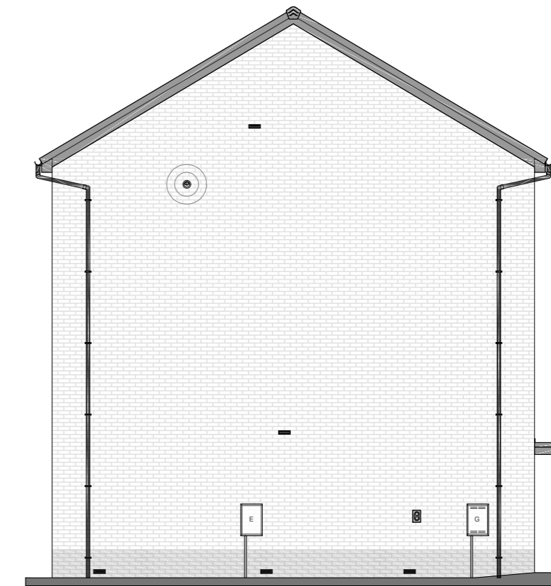
LEFT ELEVATION
