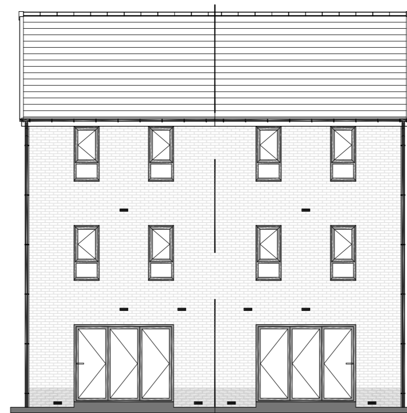
REAR ELEVATION
