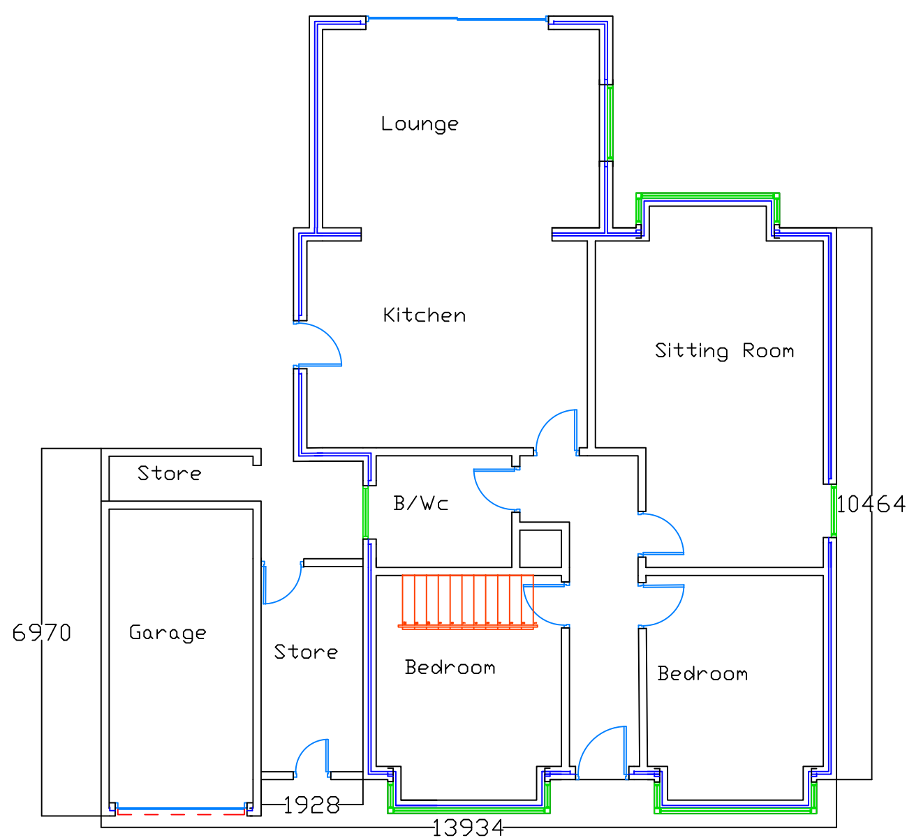
Existing Floor Plan
