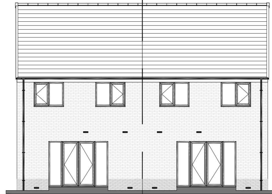
REAR ELEVATION
