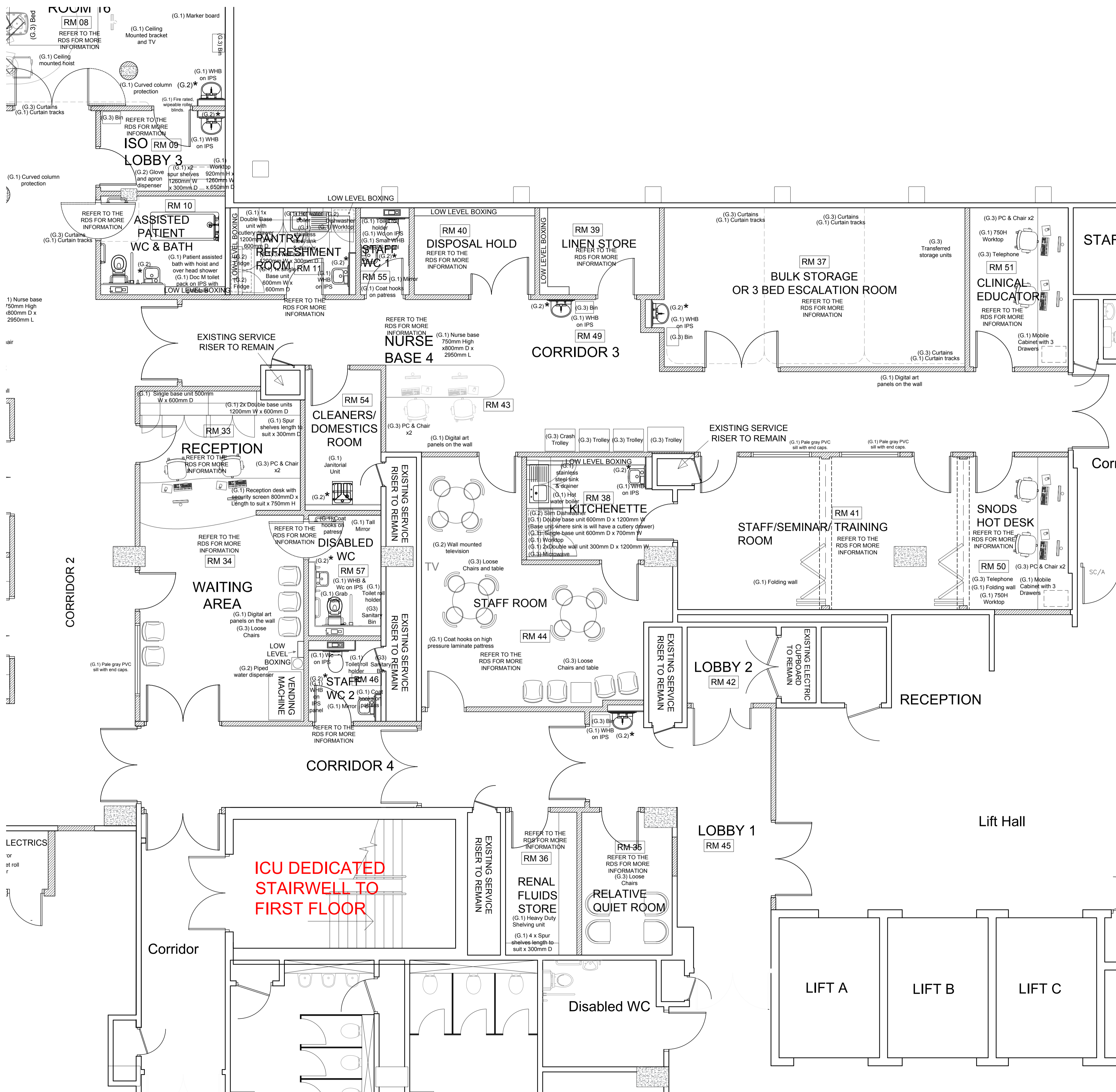
PROPOSED LOADED FURNITURE PLAN 1:100
