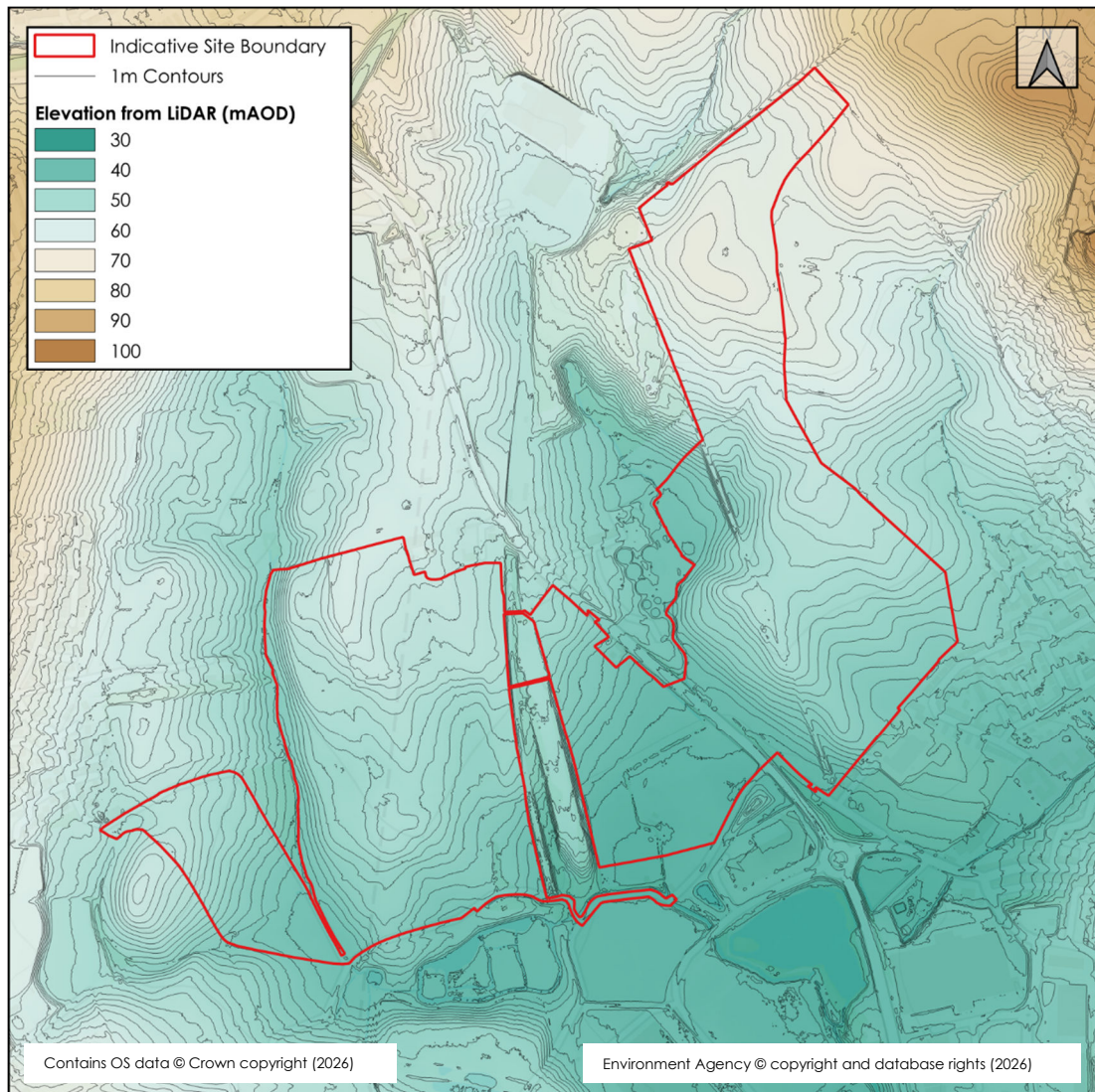
Figure 1.2: Site Topography
