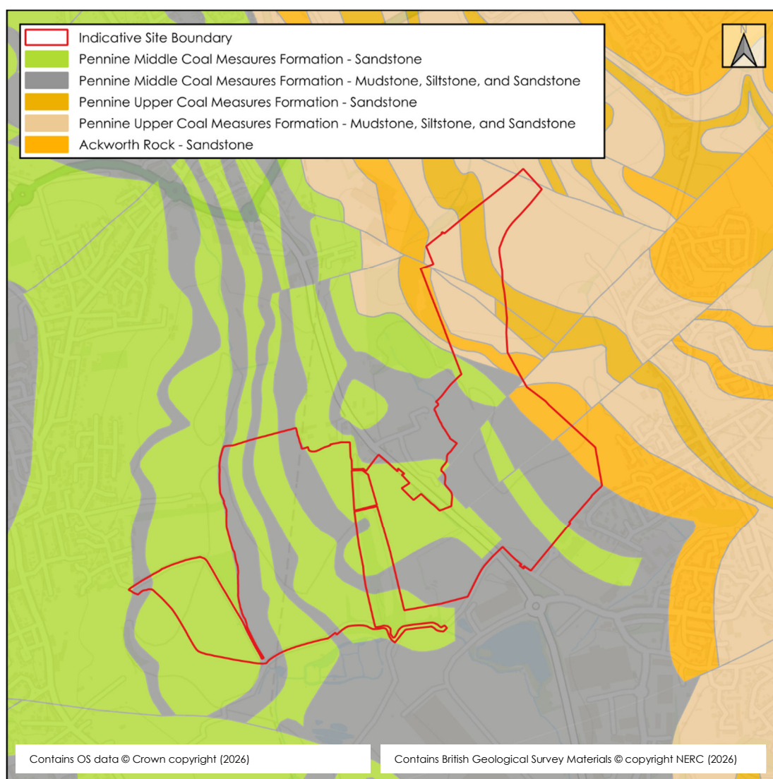
Figure 3.5: BGS Bedrock Map
