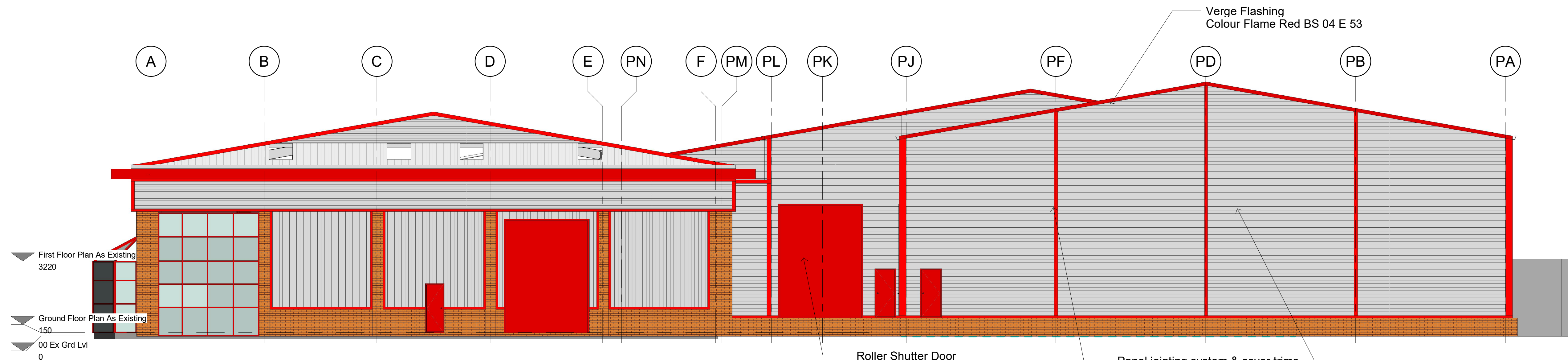
2 Elevation 2 West Landscape Omitted 1 : 100
