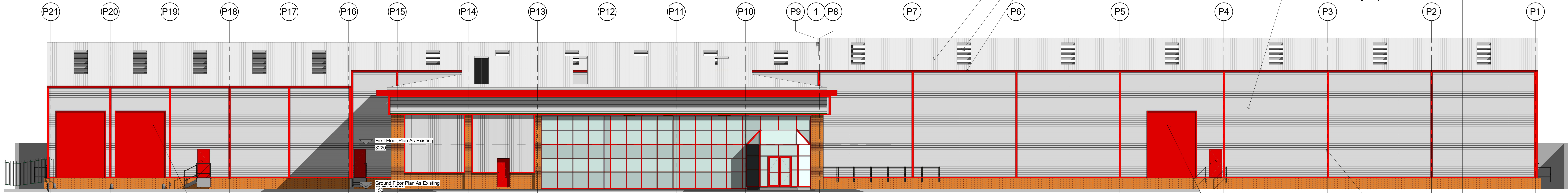
3 Elevation 3 North Landscape Omitted 1 : 100
