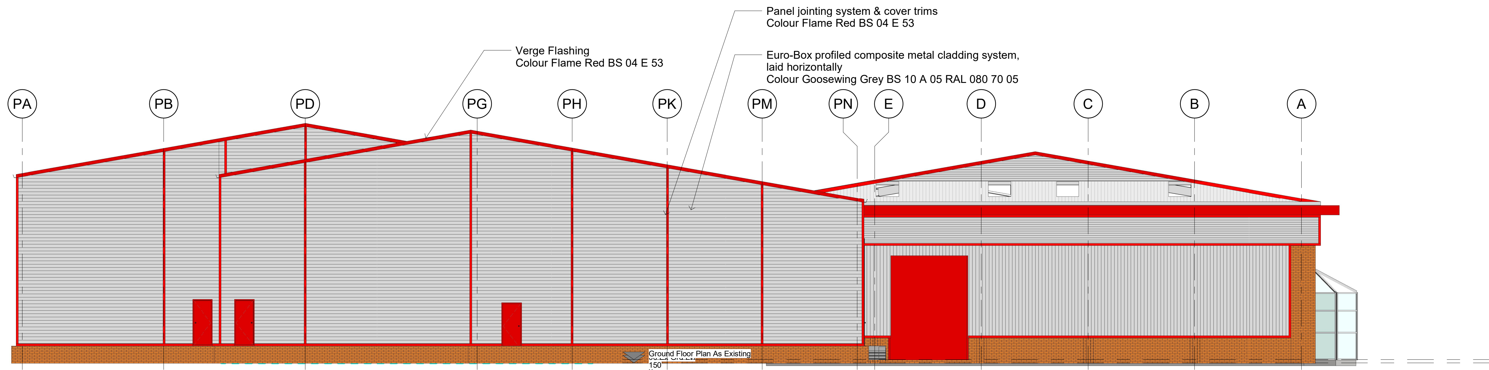
4 Elevation 4 East Landscape Omitted 1 : 100
