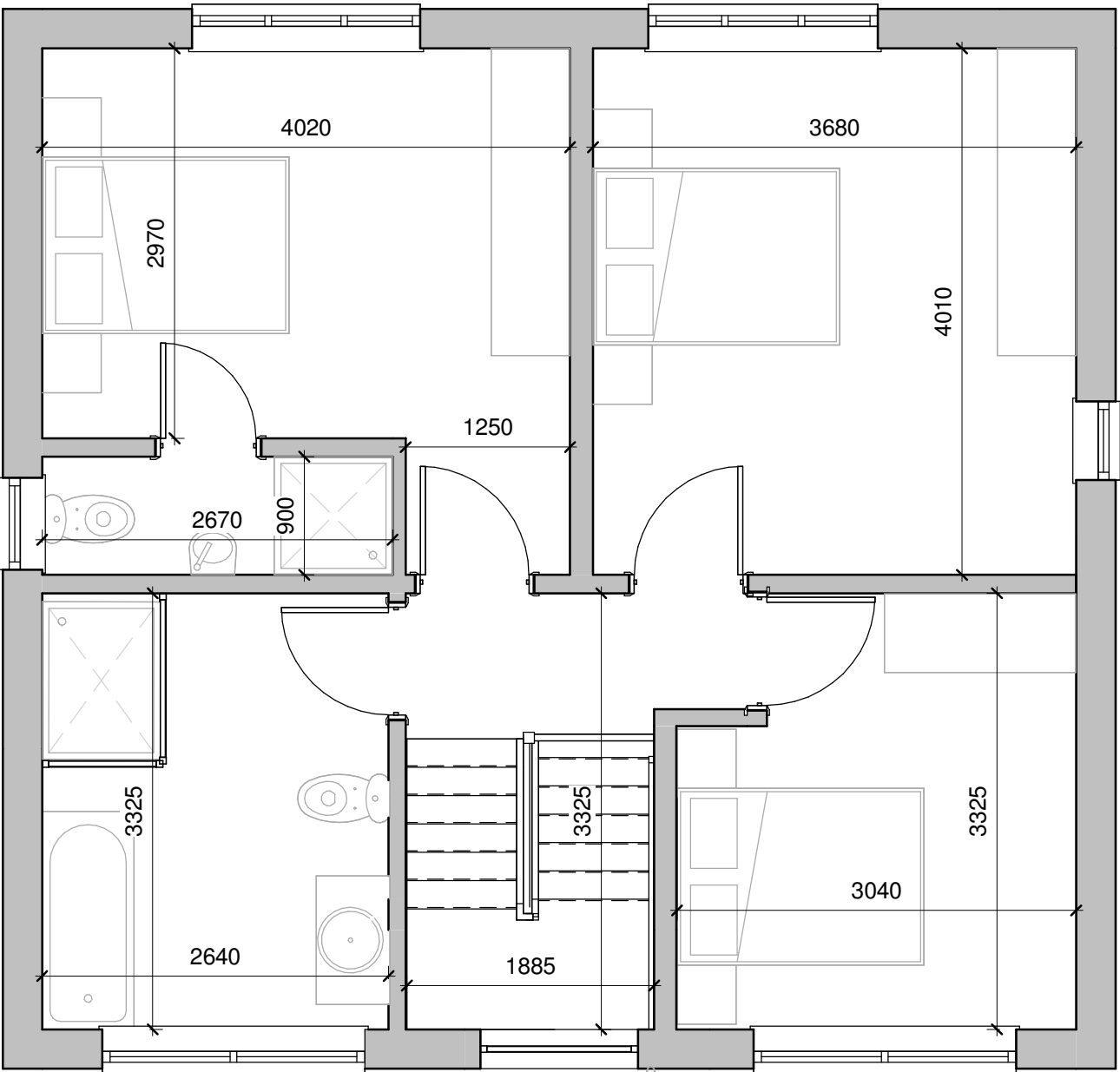
First Floor Level Dimensioned 1 : 50
