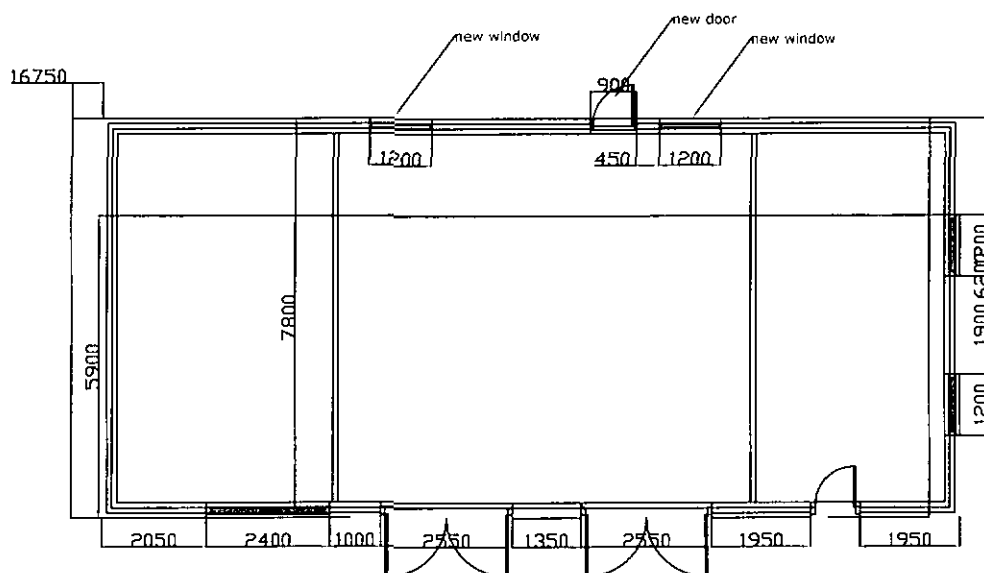
Plan as Proposed
