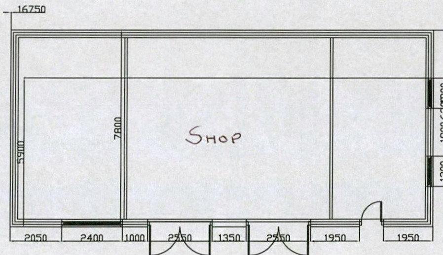
Plan as Existing
