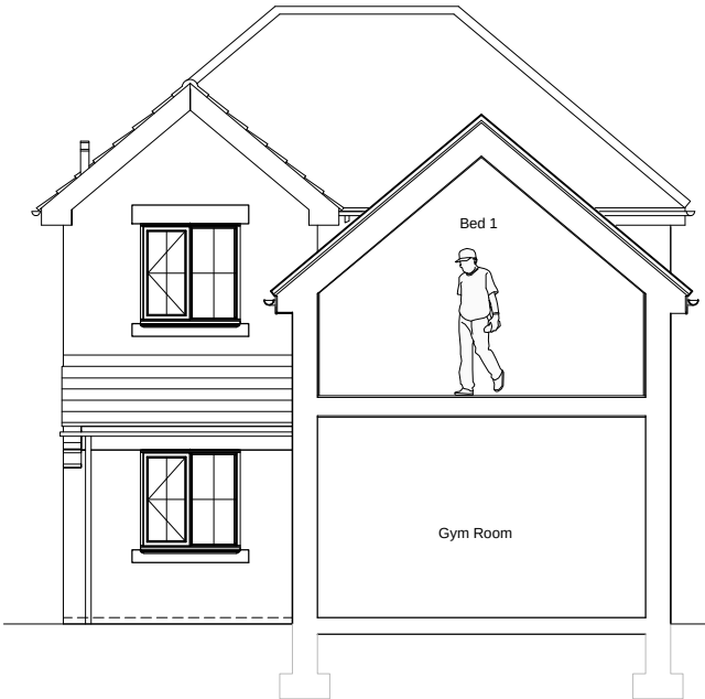
Indicative Section
