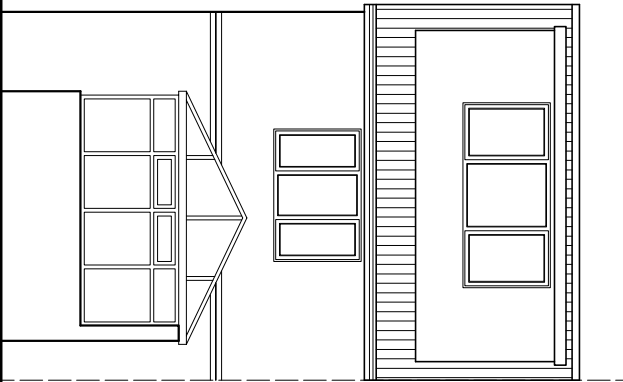
EXISTING REAR ELEVATION SCALE 1:100
