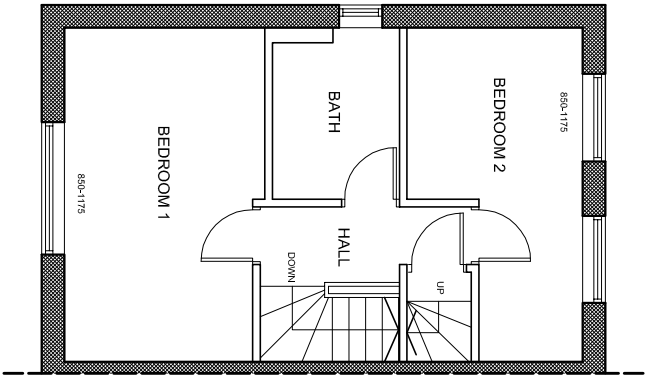
PROPOSED FIRST FLOOR PLAN SCALE 1:50
