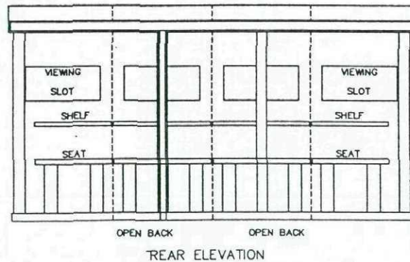
REAR ELEVATION
