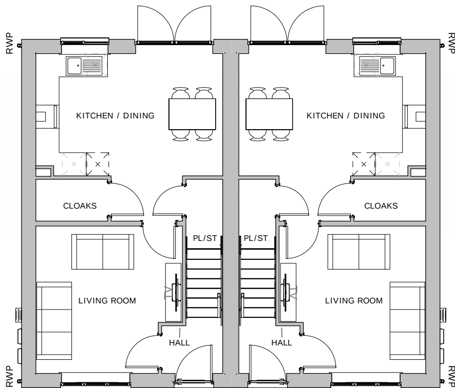
Ground Floor 1 : 100
