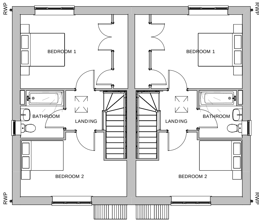
First Floor 1 : 100
