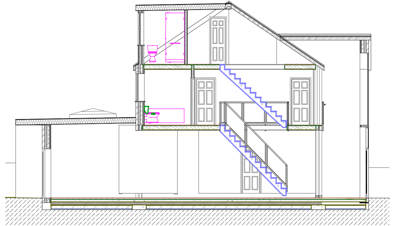
2 S-06 Building Section 1:100
